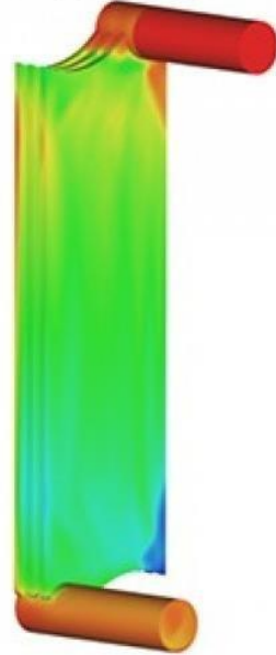
Hot domain
