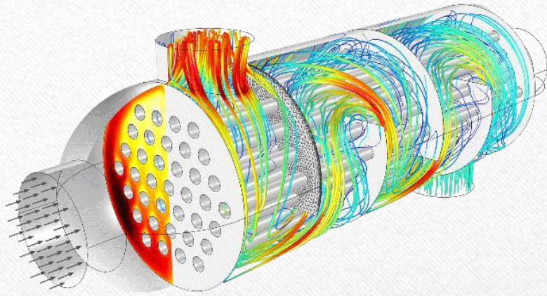
Heat Exchangers
